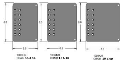
ADULT ALUMINUM ANGLE ADJUSTABLE FOOTPLATE SMALL MEDIUM LARGE
